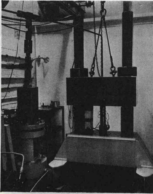
FIG. 3. 200,000 psi testing system.
